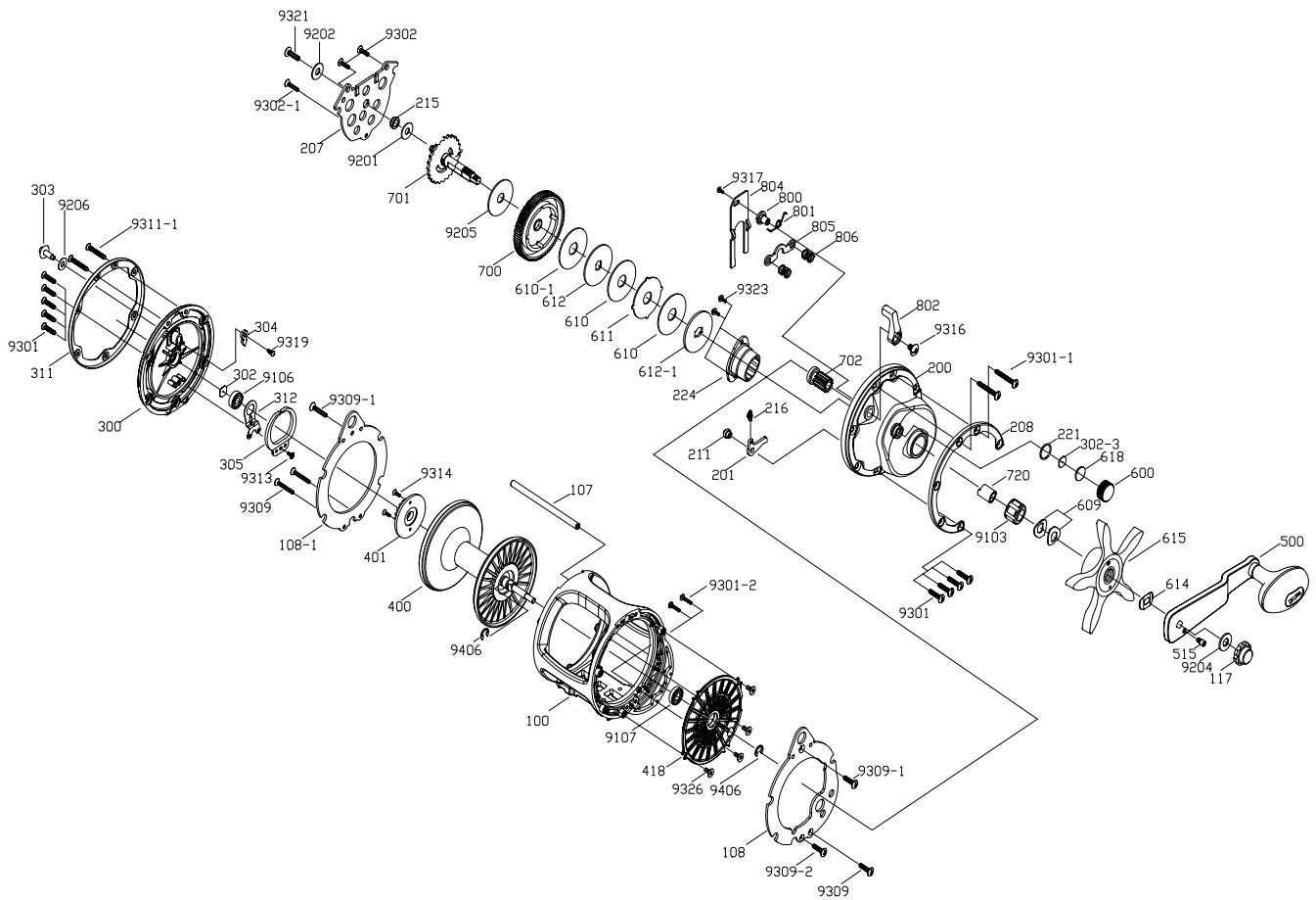
CV - 55SS Spare Parts
